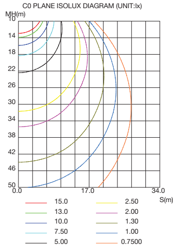
ISOLUX DIAGRAM
